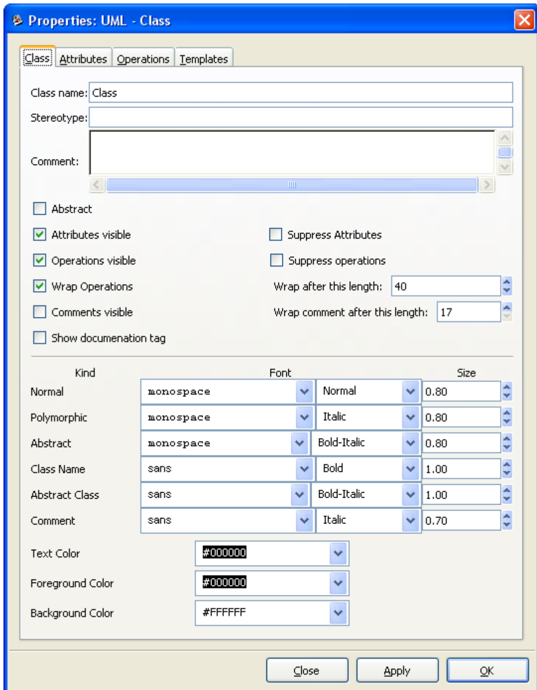
Figure 6-11. UML Class Properties
